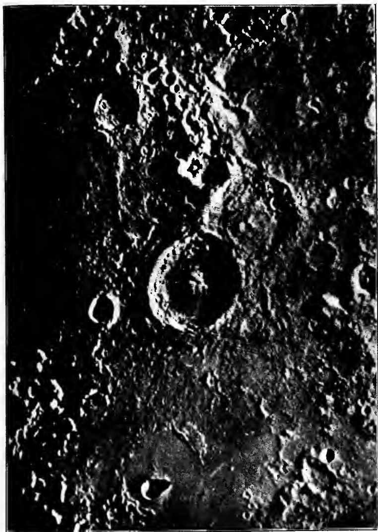
LUNAR CRATER THEOPHILUS AND SURROUNDING REGION
